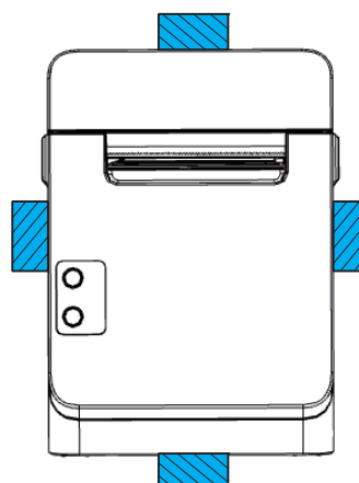
Vertical/Wall-hanging installation (Front View)
