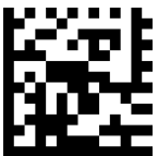
Delay 750 MS
